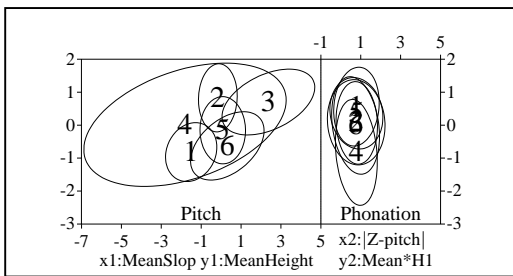
Figure 4: Pitch (left) and phonation contrasts (right) of the six tones in Ruokeng both in terms of confidence ellipses specified by two-dimensional features. The number of scatter plots for each tonal ellipse is 250.
