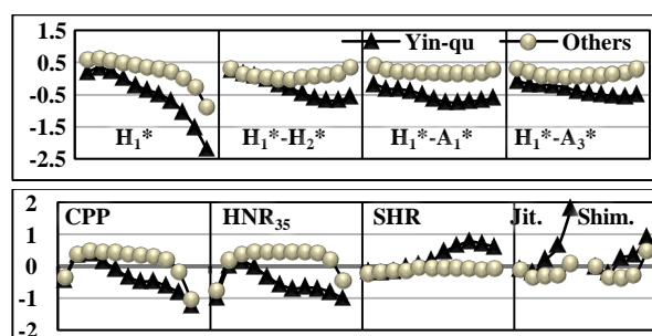
Figure 3: The 9 acoustic parametric curves for T4 (Yin-qu: black) and the mean of the other 5 tones (grey) in Ruokeng.
