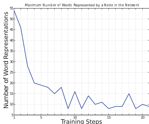
Fig. 7: The maximum number of words represented by a neuron in the network.
