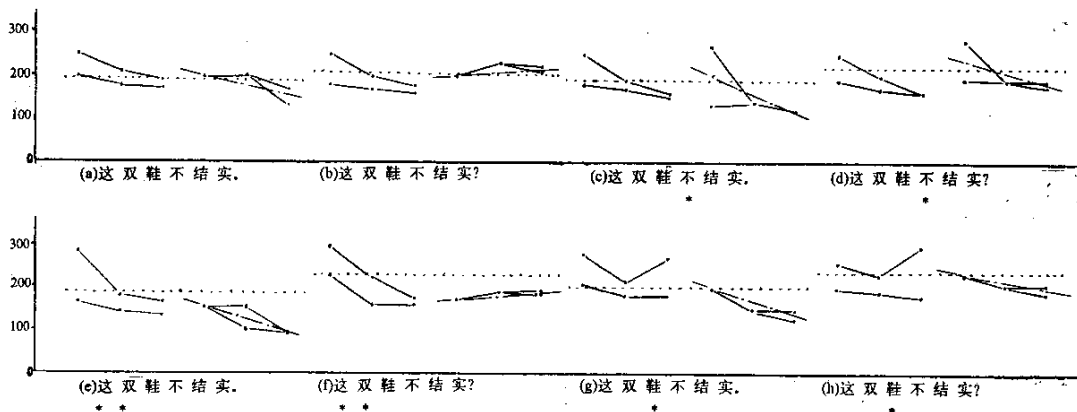
Fig. 2 (1) Dashed lines show the influence of speech mood and stress allocation upon the slope of intonation contour; (2) dotted lines show the influence of speech mood upon the whole pitch register of the sentence.
